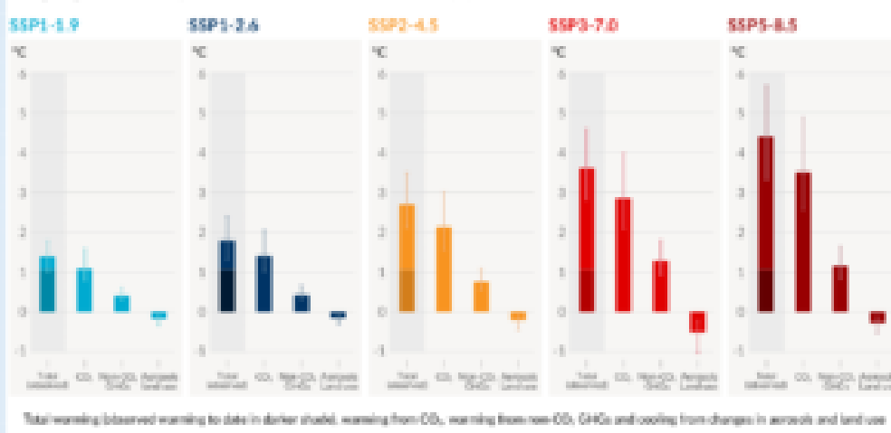
b) Contribution to global surface temperature increase from different emitters, with a dominant role of CO 2 emissions Change in global surface temperature in 2081-2100 relative to 1950-1999 (°C)
